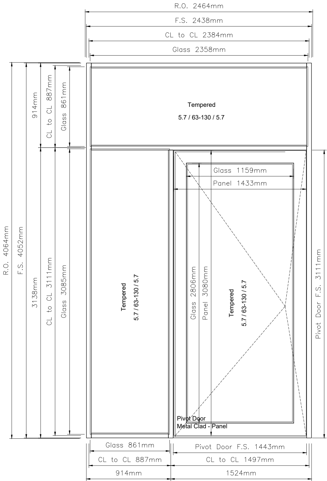
Curtain Wall with Incorporated Pivot Door
